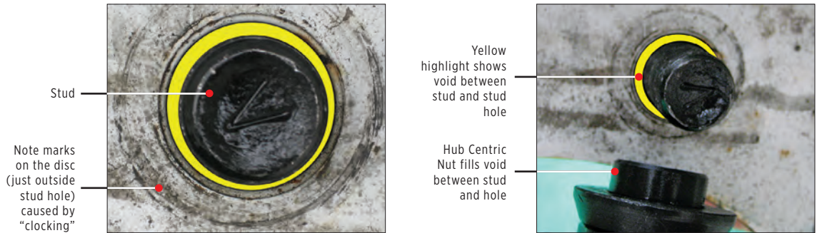
This nut had been torqued to specifications and retorqued per factory settings.
